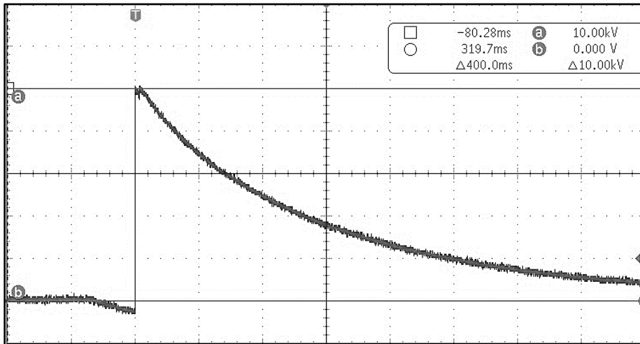
Figure 2. MegaPulse Antenna Surge PF Output Waveform
