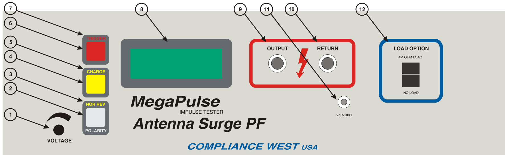
Figure 3. MegaPulse Antenna Surge PF Front Panel.
