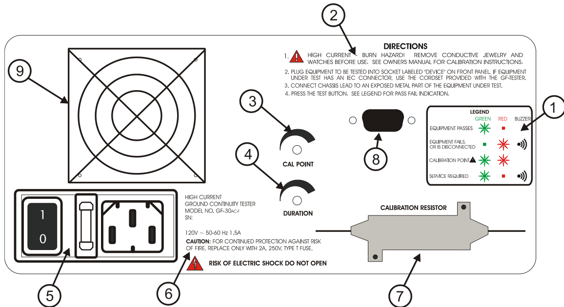
Figure 2-2. Control, Indicators, Connectors - Model GF-30AC-T Rear Panel
