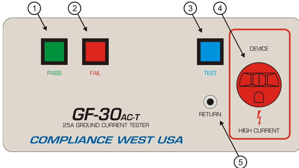
Figure 2-1. Controls, Indicators, Connectors - Model GF-30AC-T Front Panel
