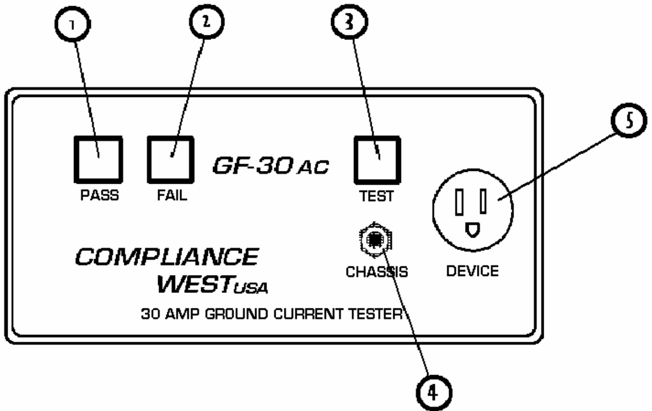
Figure 2-1. Controls, Indicators, Connectors - Model GF-30AC Front Panel
