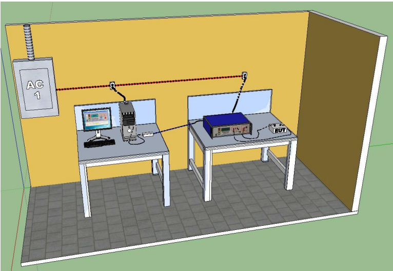
Incorrect Connection
