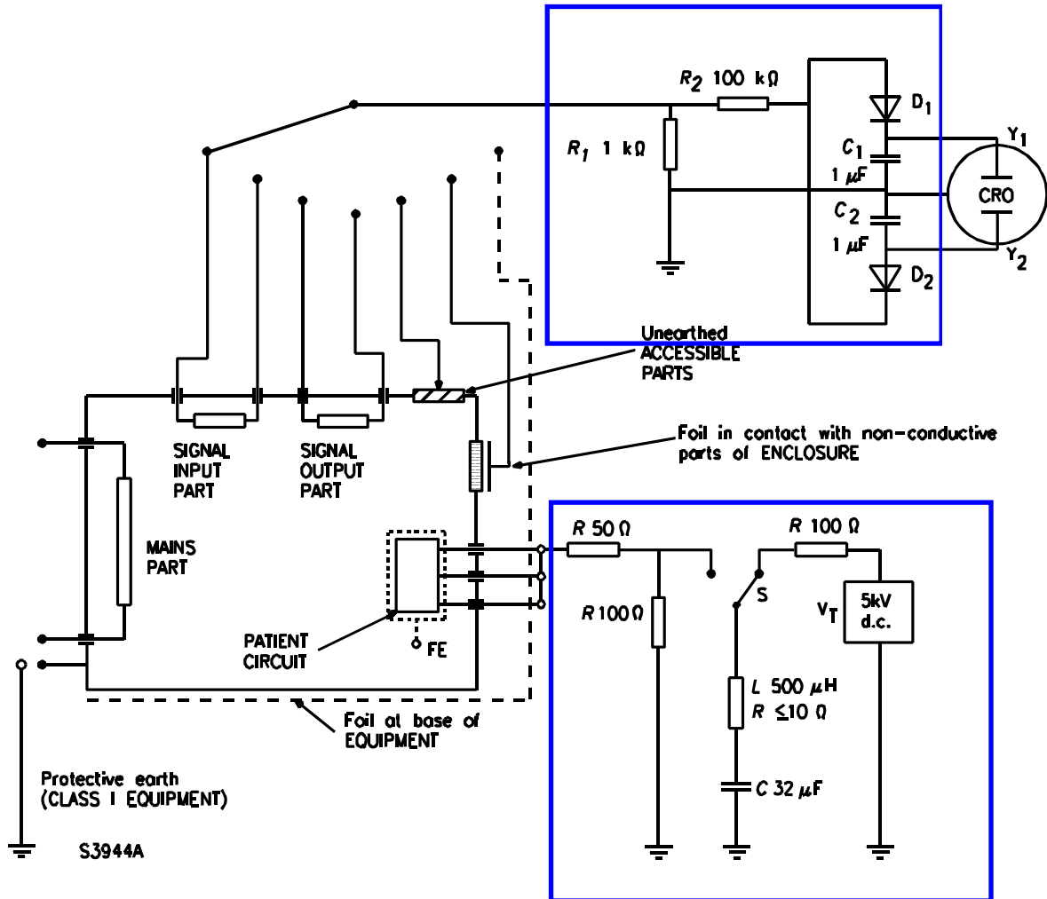
Figure 50 – Application of test voltage to bridged PATIENT CONNECTIONS for DEFIBRILLATION-PROOF APPLIED PARTS (see subclause 17 *h))
